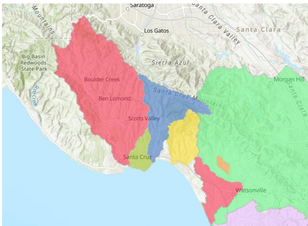
Figure 7: Map of impaired water bodies in the County as identified by the Central Coast Regional Water Quality Control Board .
